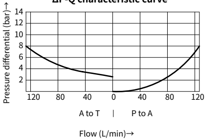
\Delta P -Q characteristic curve
